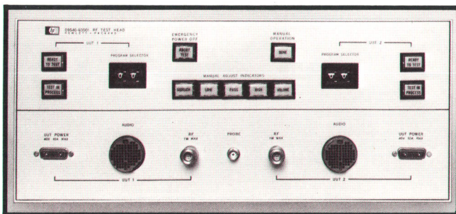
Fig. 4. Transceivers to be tested are connected to this RF test head. Two units at a time can be connected; one can be warming up while the other is being tested. A 15-foot cable allows the test head to be inside a screen room while the system remains outside.
